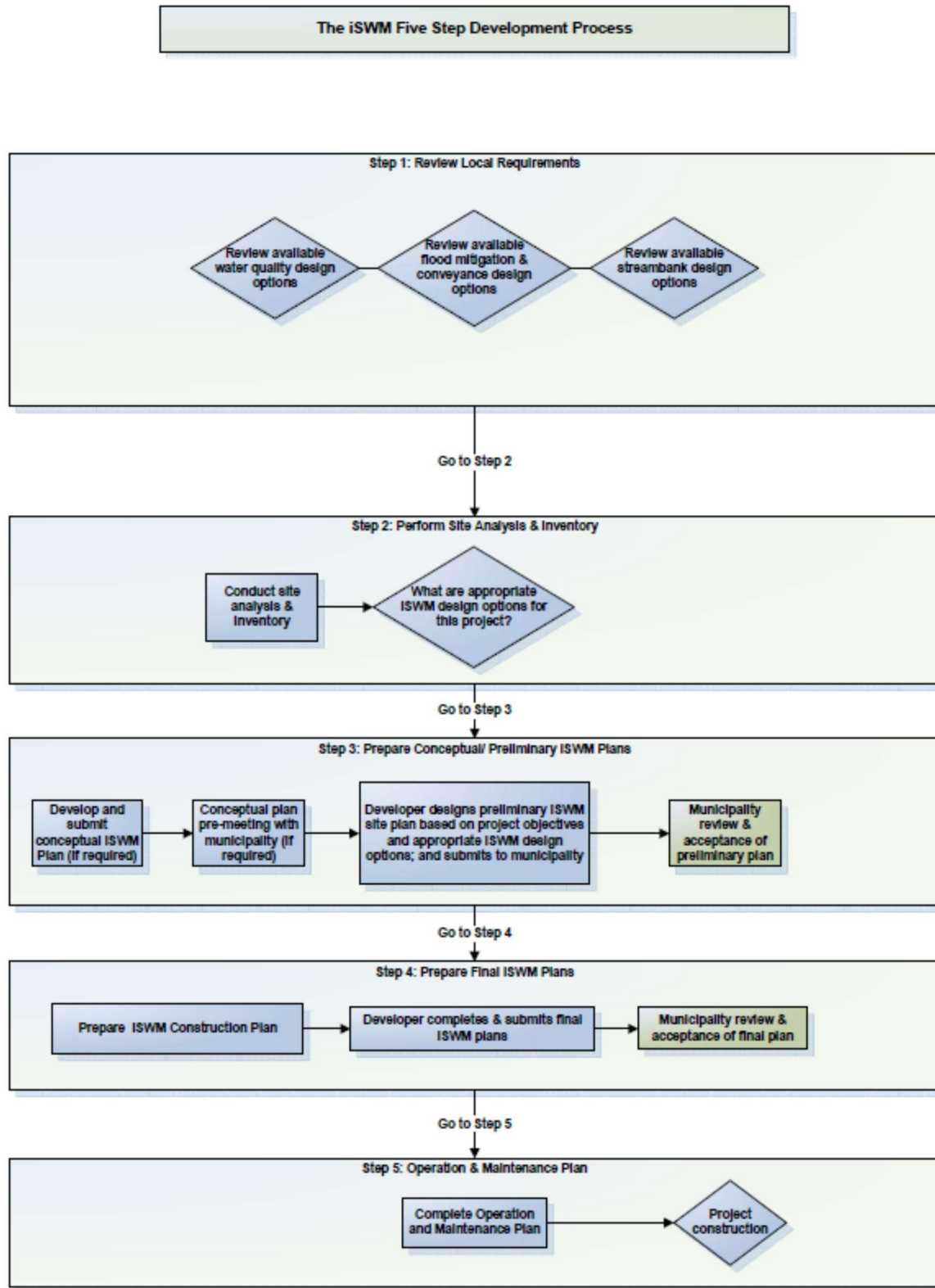
Figure 2.1 iSWM Flowchart
